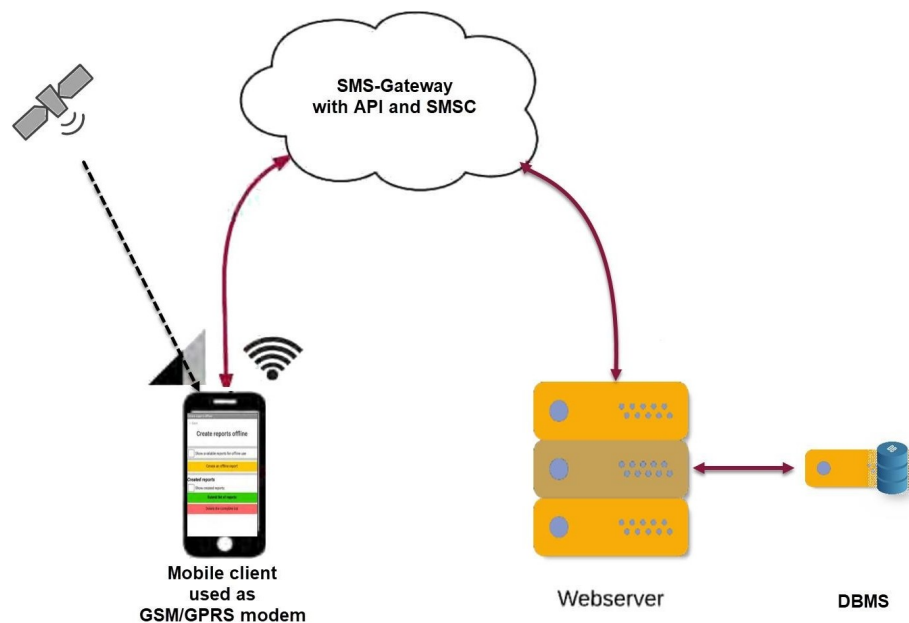
Fig. 3. Communication flow when creating and submitting a report using SMS.
